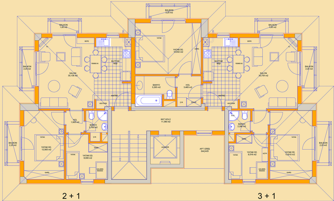
NORMAL KAT PLANI 1/50
